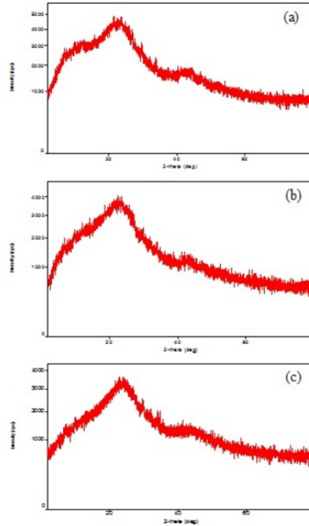
Figure 3: XRD pattern with blender time variation (a) without blender (b) 30 minutes (c) 60 minutes.
